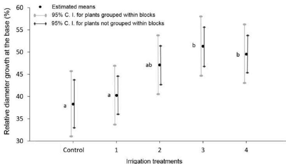
Figure 5. G.L.M.M. estimated marginal means of the relative diameter growth at the base (%) by irrigation treatments, with plants grouped or not within blocks. Different letters denote statistically significant differences at the 5% level without grouping plants within blocks as a random factor.
