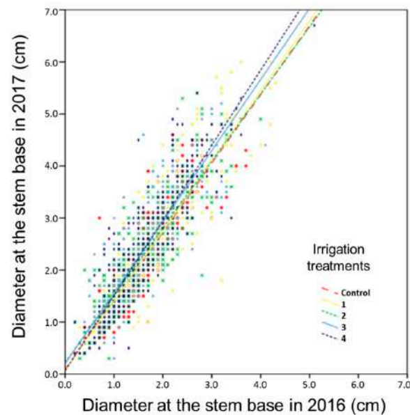
Figure 4. Linear relationship between initial (2016) and final (2017) diameter at the base, separated by irrigation treatments.
