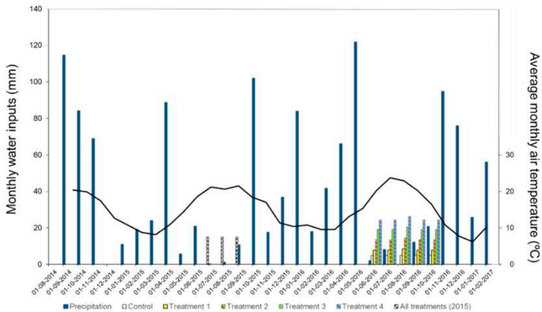
Figure 2. Ombrothermic chart of monthly rainfall and mean temperature that occurred in the experimental plot since planting, including monthly irrigation water inputs per treatment. Control received survival irrigation.
