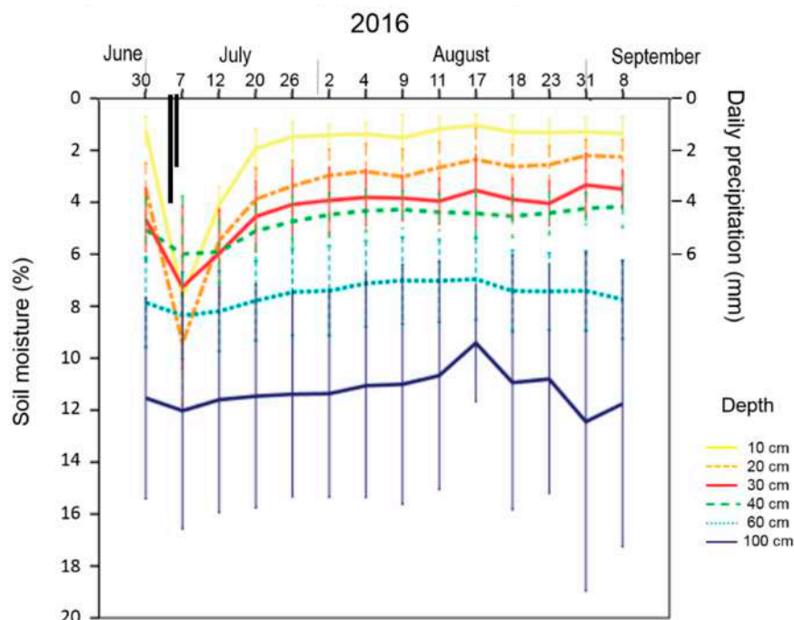
Figure 3. Average (lines) and standard deviation (vertical lines) of instantaneous soil moisture measured at six depths in all the locations from the experimental plot, and daily precipitation (black bars) during summer 2016.
